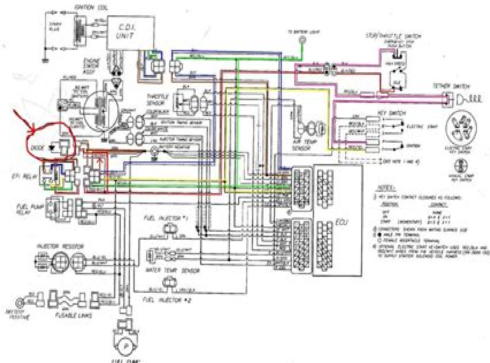
Wiring Diagram (EFI System Harness)
