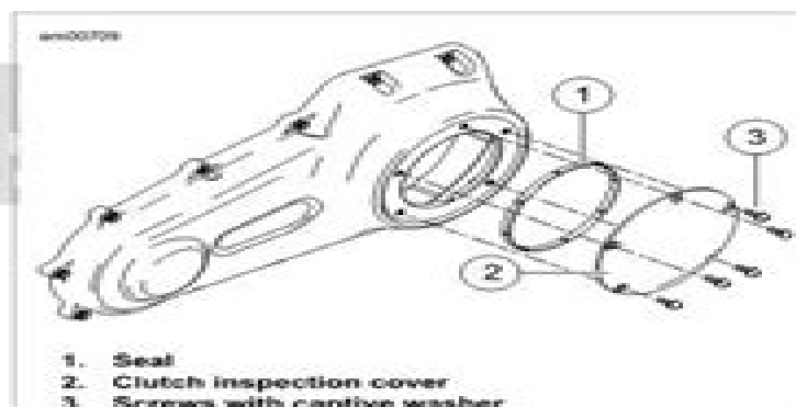
Figure 1-9. Clutch Cover
