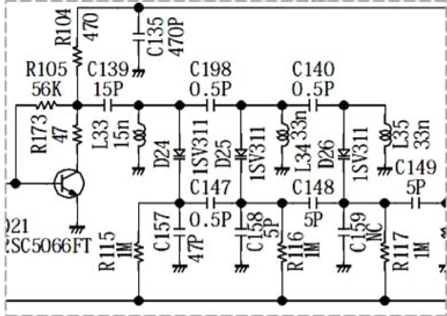
Preview: ALINCO DJ-C7T schematic diagram
