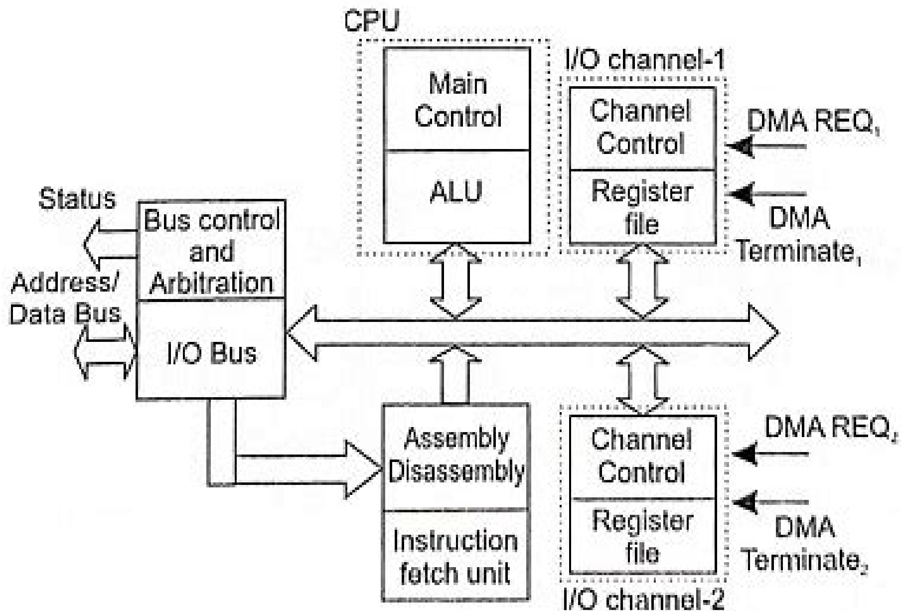
Fig. 9.104 Block diagram of 8089 I/O processors
