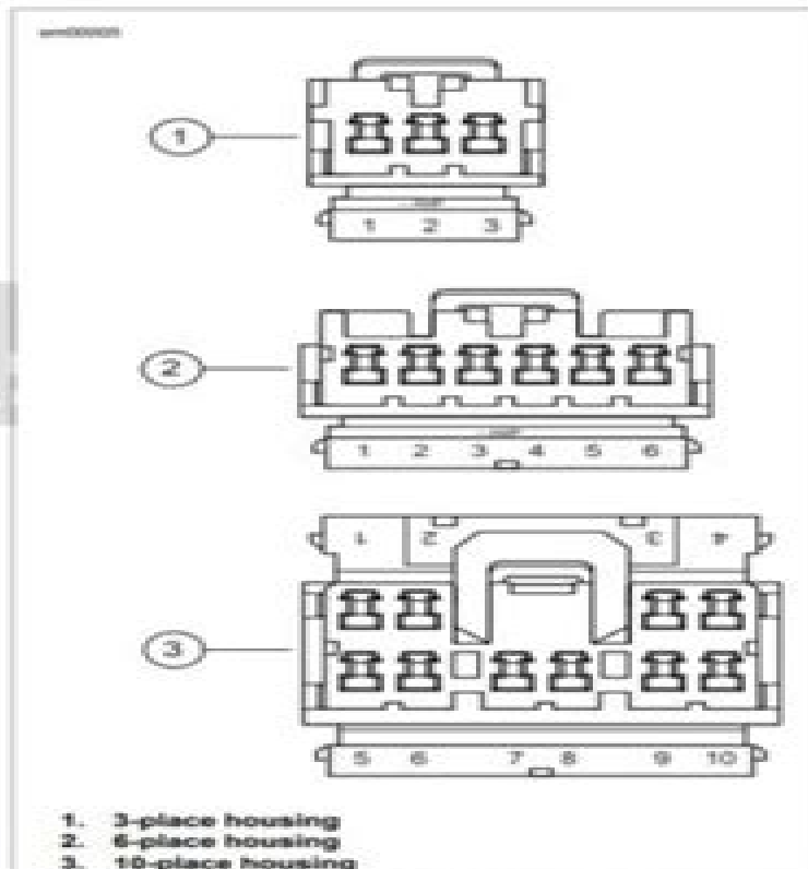
Figure A-57. Tyco 970 Multilock Unsealed Connector: Cavity Numbers on Secondary Locks (socket housings shown)
