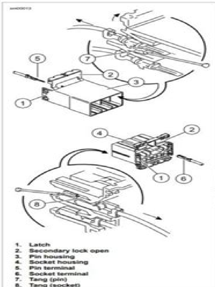
Figure A-56. Tyco 970 Multilock Unsealed Connector: Socket and Pin Housings
