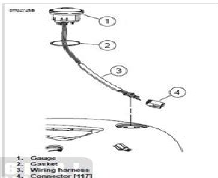
Figure 7-69. Fuel Gauge
