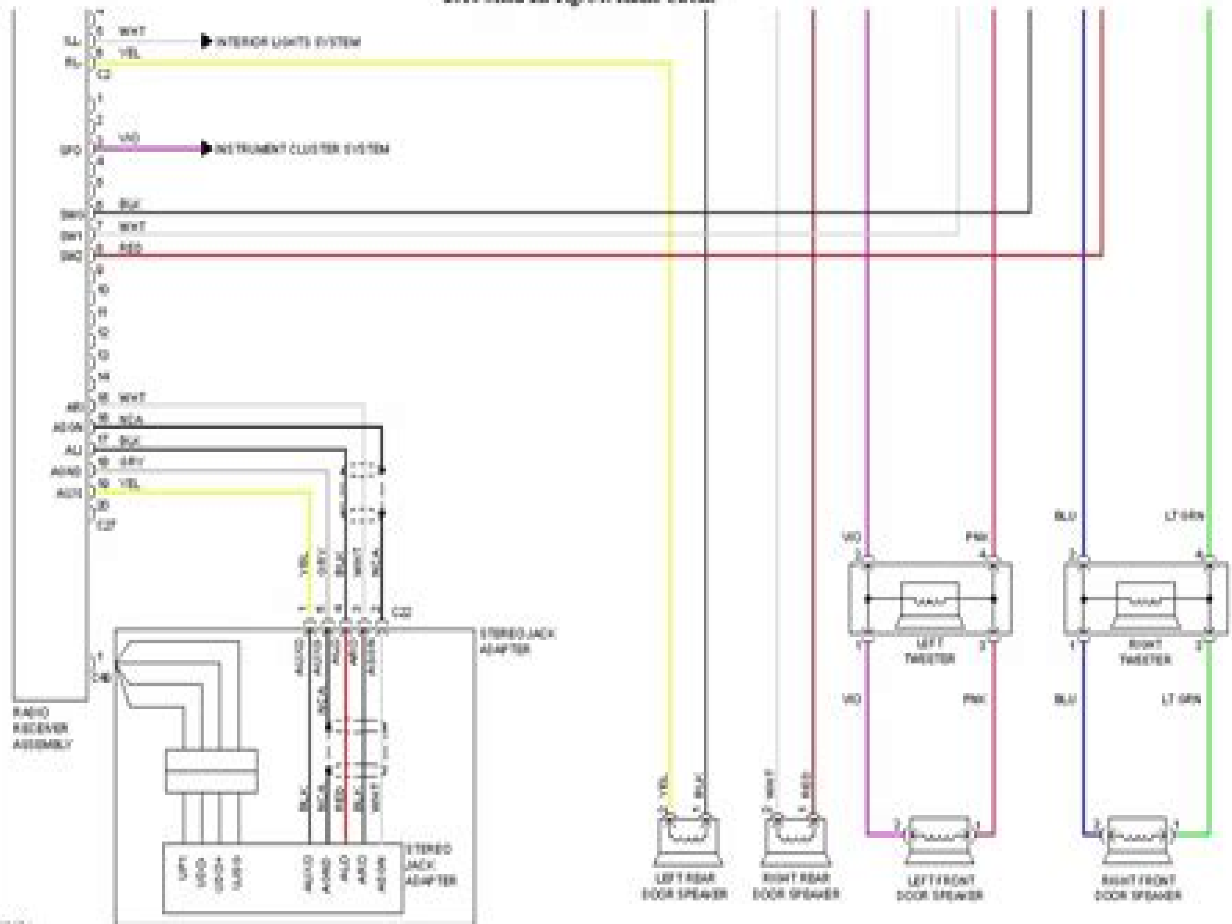
2010 Scion xB-Fig. 34: Radio Circuit
